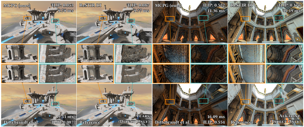
Fig. 8. Roughly equal-time renders, comparing the effectiveness of direct light rendering with the the screen-space technique of Dittebrandt et al. [2023] and the unbiased MIS variant of ReSTIR DI [ Bitterli et al. 2020 ] using one temporal and four spatial reuse passes. Our method demonstrates competitive performance in terms of both execution time and approximation error in environments characterized by simple guiding distributions (left). However, it exhibits limitations in scenarios with many light sources (right) compared to ReSTIR. Nonetheless, our method is capable of adapting its distribution to prioritize the most significant light sources, thereby delivering a temporally stable output.
