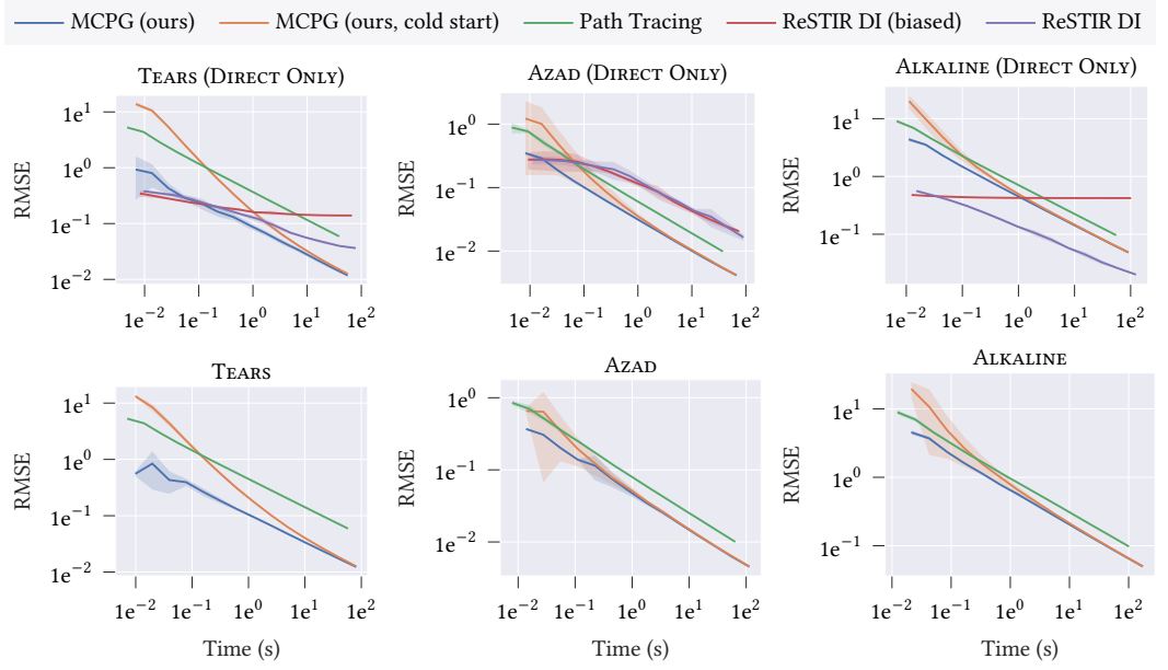
Fig. 5. Accumulation error (root mean squared error) for three of our scenes. We compare our estimator with (blue) and without (orange) warm-up phase against path tracing with BSDF importance sampling and ReSTIR DI. ReSTIR DI can only be used for estimating direct light (top row). The bottom row shows errors for two-bounce indirect lighting. Our guiding distribution usually converges within 100 frames. In TEARS and AZAD, ReSTIR DI suffered from outlier samples and correlation artifacts, slowing down convergence.
